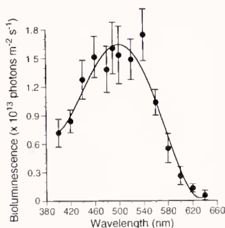
Figure 9. Behavioral spectral sensitivity of Sergestes similis based on the bioluminescence spectral efficiency, corrected for a stimulus irradiance of 1.2 \times 10^{13} photons m^{-2} s^{-1} (see text). Symbols represent means \pm SE for 9 specimens; the curve is a fourth degree polynomial function fitted to the data, where y = 6.1 \times 10^{-4}x^4 - 1.2 \times 10^{-6}x^3 + 9.2 \times 10^{-10}x^2 - 3.0 \times 10^{-13}x + 3.6 \times 10^{-15} .
